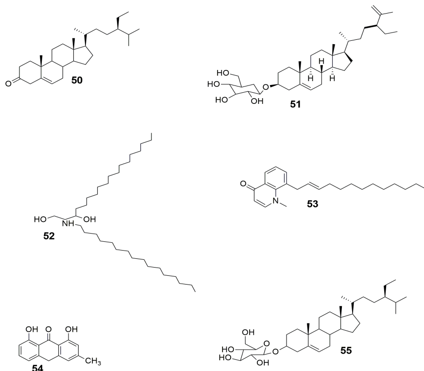
Figure 5. Chemical Structures isolated from different parts of Newbouldia laevis . \beta -sitosterone (50), stigmasterol glucoside (51), hexadecadihydrospingosine (52), evocarpine (53), chrysarobin (54), harmalol (55).
