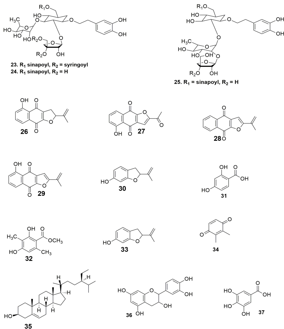
Figure 3. Chemical Structures isolated from different parts of Newbouldia laevis . Newbouldiosides D-F (23-25), 5-hydroxy-dehydroiso- \alpha -lapachone (26), 2-acetyl-5-hydroxynaphtho[2,3- \beta ]furan-4,9-dione (27), 2-isopropenyl-naphtho[2,3- \beta ]furan-4,9-dione (28), 2-(1'-methylene)-5-hydroxynaphtho[2,3- \beta ]furan-4,9-dione (29), 2-(1'-methylene)-7-hydroxy-naphtho[2,3- \beta ]furan-4,9-dione (30), \beta -resorcylic acid (31), atraric acid (32), 2-(1'-methylene)-6-hydroxy-2,3-dihydrobenzo[ \beta ]furan (33), 2,3-dimethoxy-1,4-benzoquinone (34), \beta -sitos-terol (35), epicatechin (36), gallic acid (37).
