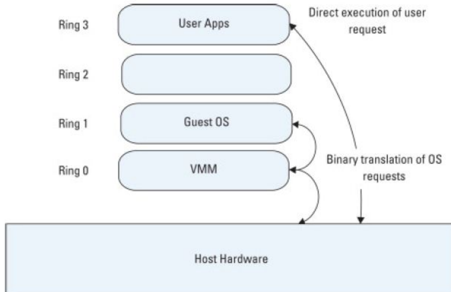
Fig. 4. Full Virtualization
