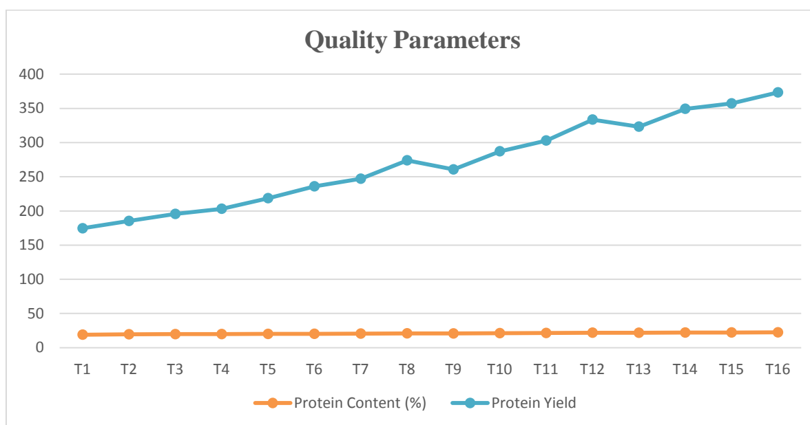
Fig. 3. Effect of quality parameters of lentil as influenced by phosphorous and boron levels
