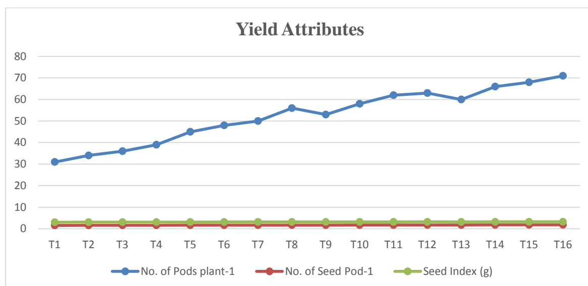
Fig. 1. Effect of yield attributes of lentil as influenced by phosphorous and boron levels
