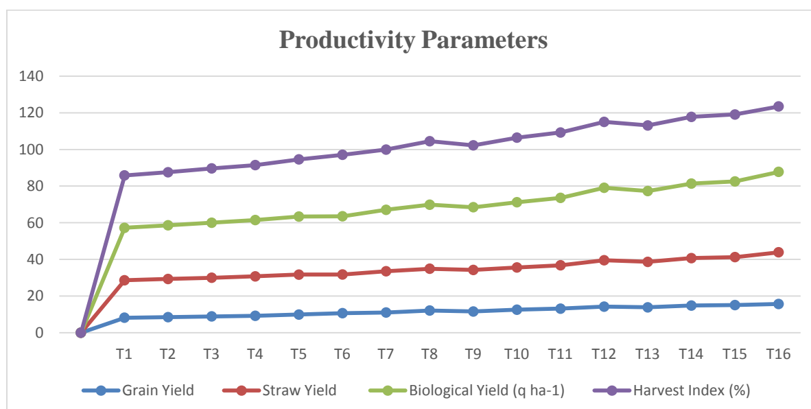
Fig. 2. Effect of productivity parameters of lentil as influenced by phosphorous and boron levels
