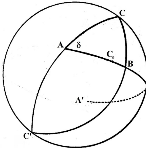
Fig. 2. The phase \angle C'AB is determined by the angle excess of the triangle BAC collinear to C'AB . As B \rightarrow C , the two beams will have opposite phases, while as B \rightarrow C' , which is the opposite state of polarization to C , the phase will vanish.
