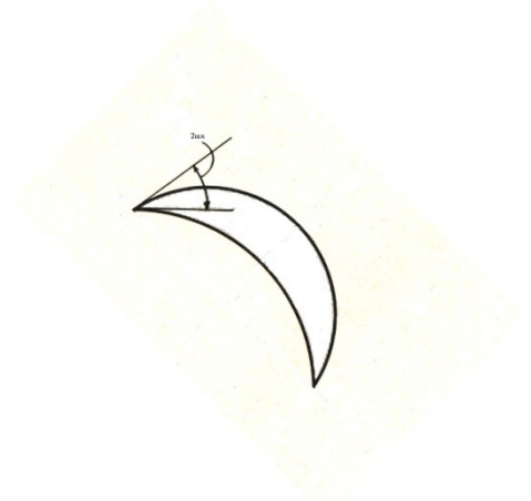
Fig. 3. Two circular arcs intersect at an angle 2\alpha\pi .
