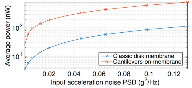
Figure 7. Simulated power response of the classic and the proposed topologies when subjected to band-limited white noise (10 Hz to 2 kHz).
