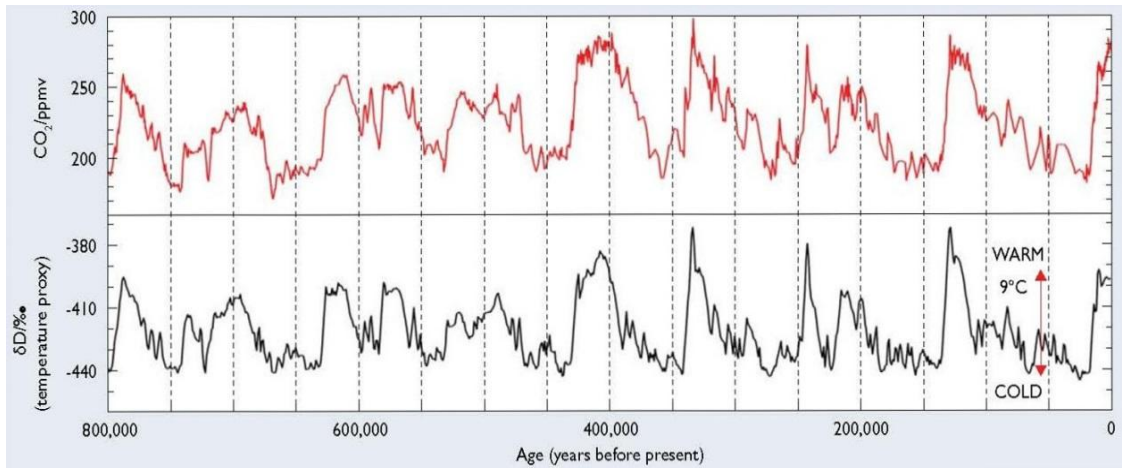
Fig. 4. Correlation between local temperature and trapped CO 2 over a time span of 800,000 years from an Antarctic ice core: Ice core data from the EPICA Dome C (Antarctica) ice core: deuterium is a proxy for local temperature; CO 2 is from the ice core air. Data from [60,61]. Reproduced with permission of the British Antarctic Survey
