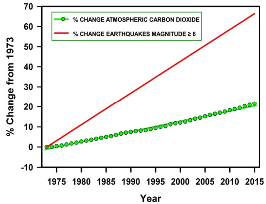
Fig. 3. Percent annual change, relative to 1973, of earthquakes, magnitude ≥ 6, shown by the regression line from Fig. 1, and from CO 2 values based on the model-based tabulation published by NASA Goddard Institute for Space Studies (GISS) [58]. This figure shows that earthquakes of magnitude ≥ 6 are increasing at a greater rate than atmospheric CO 2 . Prior to 1973 earthquake data is insufficiently robust to be reliably compared with CO 2 data
