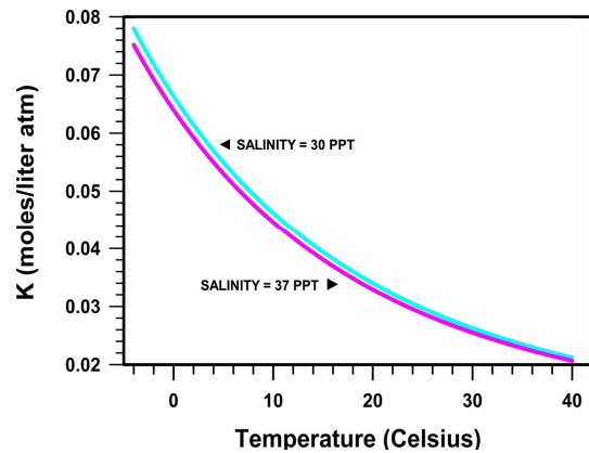
Fig. 2. The CO 2 solubility coefficient, K 0 , calculated with equation (3) throughout the entire range of temperatures and salinities, bracketed by the two extreme salinities, relevant to seawater. This figure shows that an increase in temperature, over all ocean conditions, leads to a decrease in CO 2 solubility
