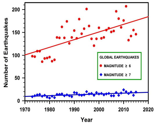
Fig. 1. The annual number of magnitude ≥ 6 and ≥ 7 earthquakes globally, taken from the U. S. Geological Survey database [50], are shown with linear regression fit lines. Regression lines (slope, y-intercept, R 2 ): For the ≥ 6 magnitude data set (1.672, -3193.1, 0.4495) and for the ≥ 7 magnitude data set (0.1799, -344.79, 0.3524). This figure clearly shows that there has been a dramatic increase in the annual number of global earthquakes in the indicated magnitude ranges over the time interval 1973-2015. For earthquakes of magnitude ≥ 6, the increase is 66%; for earthquakes magnitude ≥ 7, the increase is 74%
