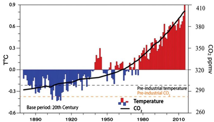
Fig. 10. Time series of annual values of global mean temperature anomalies (red and blue bars) in degrees Celsius, and carbon dioxide concentrations at Mauna Loa, both from NOAA. Data are relative to a baseline of the 20th century values. From Yan et al. [71]
