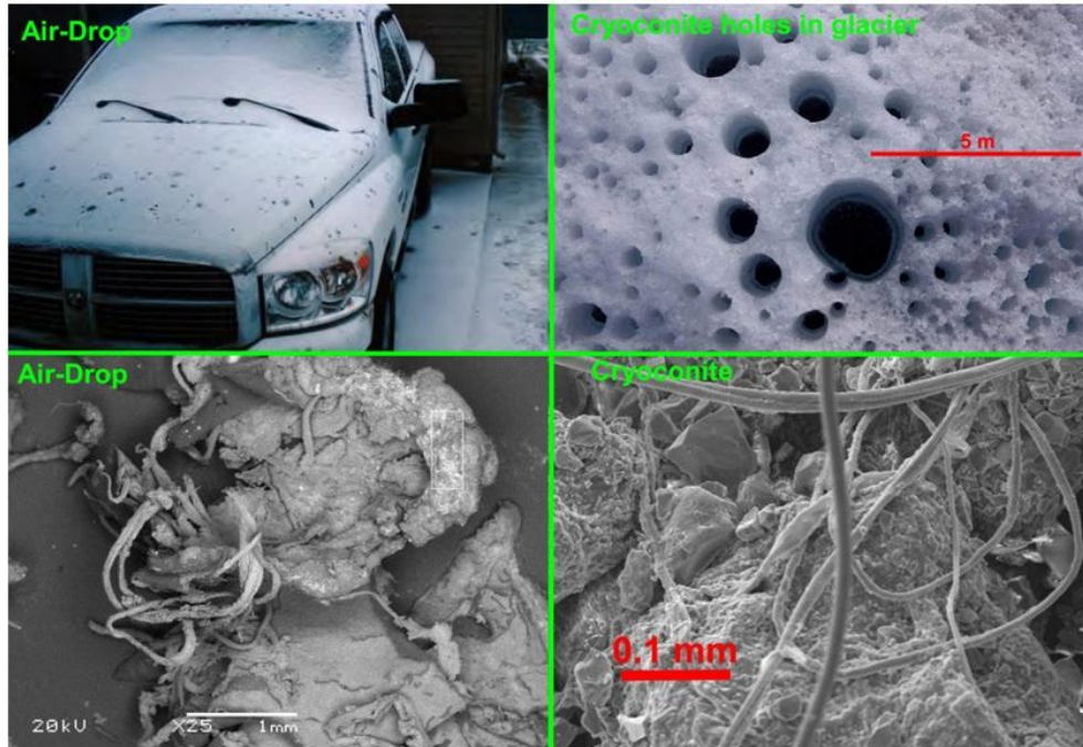
Fig. 9. Upper Left: Air-Drop Distribution; Upper Right: Cryoconite-hole Distribution in Glacier; Lower Left: Air-Drop Pseudo- or Proto-Cryoconite; Lower Right: Natural Cryoconite. Adapted from [70]
