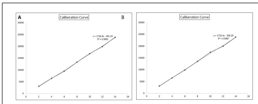
Fig. 3. Linearity calibration curves of TH in acetonitrile: water (65:35) (A) and acetonitrile: NSF (60:40) (B) respectively
