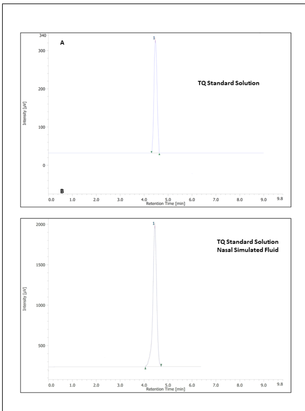
Fig. 2. HPLC chromatogram of 20-µL injection of TH in acetonitrile: water (65:35) (A) and acetonitrile: NSF (60:40) (B) respectively
