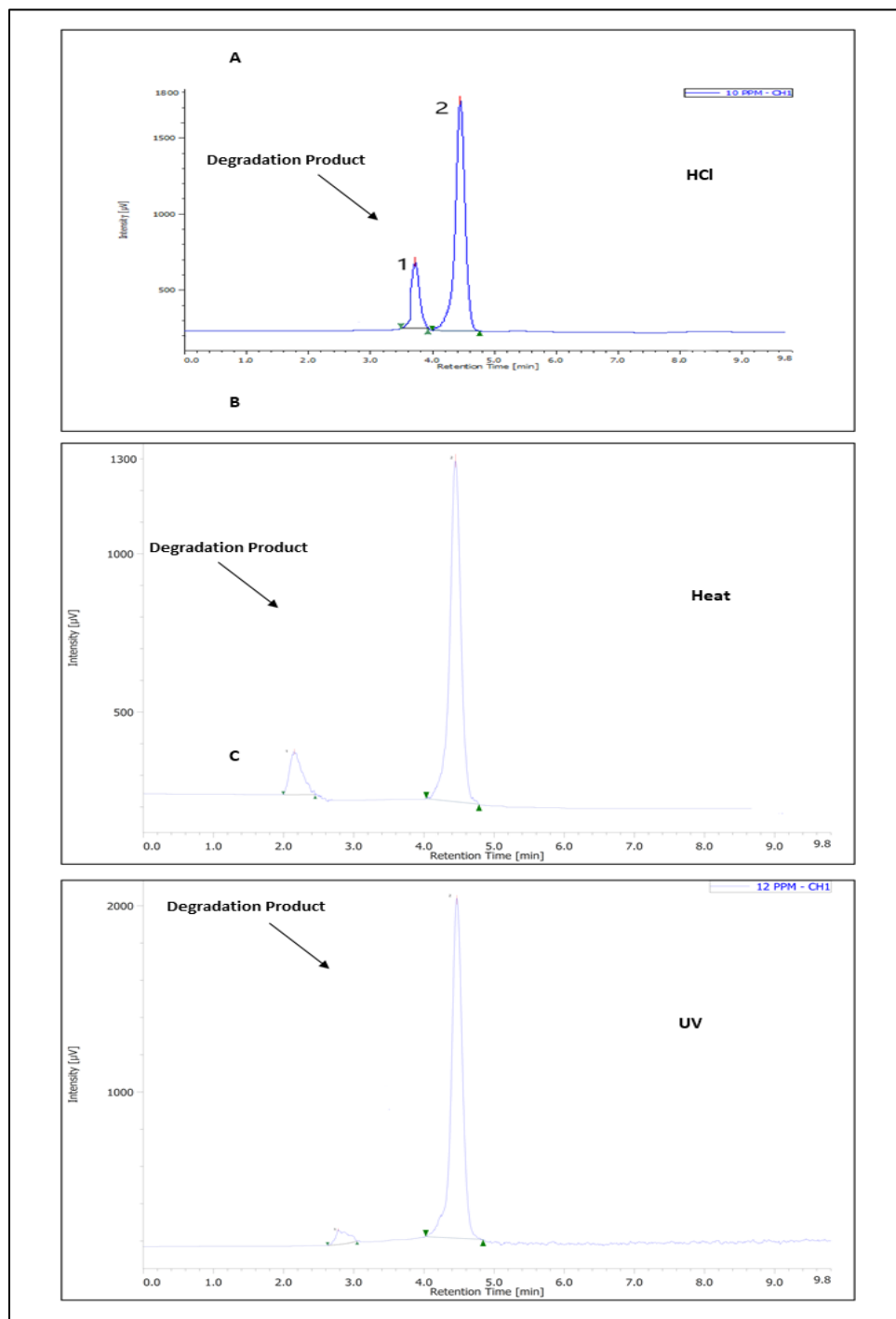
Fig. 4. Chromatograms of TH under stress conditions (A) 1 M hydrochloric acid, (B) thermal degradation, (C) photodegradation
