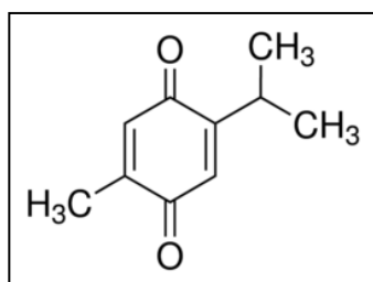
Fig. 1. Structure of Thymoquinone [7]
